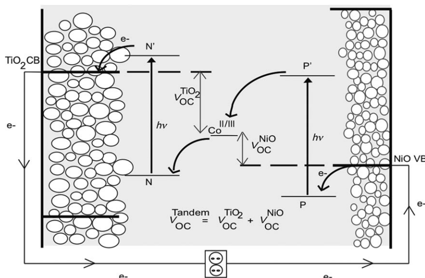
Figure 1. Schematic representation of a tandem dye-sensitized solar cell (TDSC). \text{TiO}_2 CB and NiO VB represent the Fermi level in the conduction band of \text{TiO}_2 and the valence band of the NiO, respectively; N and N', P and P' represent the energetics of the sensitizers; \text{Co}^{\text{II/III}} represents the redox potential of the electrolyte.
