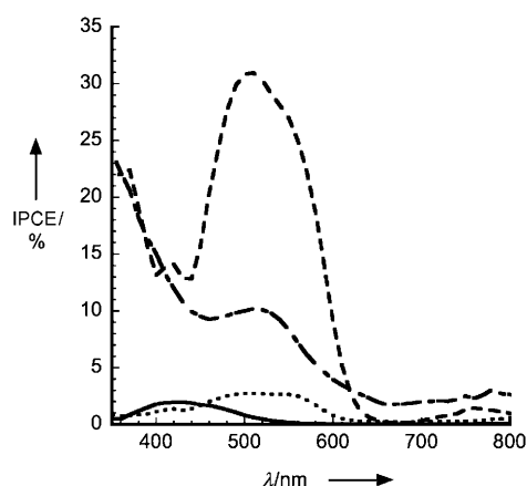
Figure 2. Incident photon-to-current conversion efficiency (IPCE) spectra of C343 (—), PI (.....), and PINDI (----) on NiO; N719 on \text{TiO}_2 (-.-.-) in the presence of cobalt-based electrolyte. Film thickness of NiO and \text{TiO}_2 were 5 \mu\text{m} and 1.5 \mu\text{m} , respectively.
